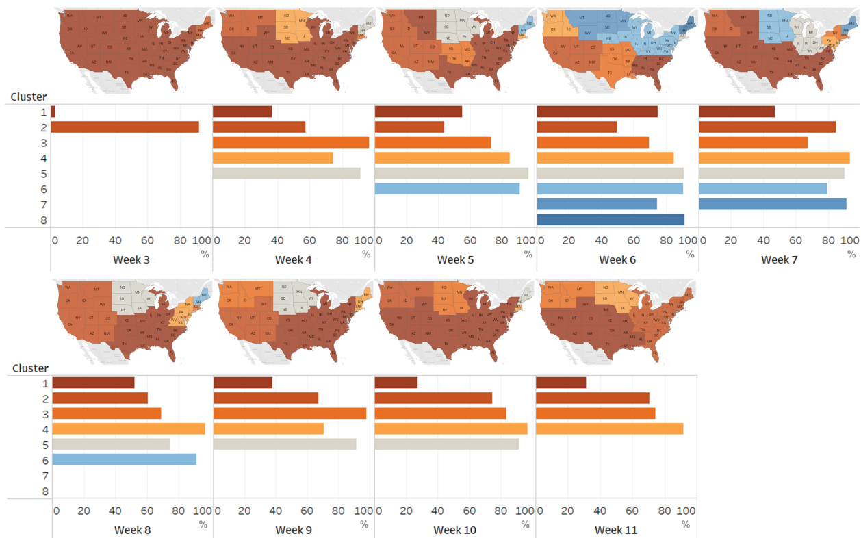
FIGURE 2: Clustering results starting from the week of March 16 and ending at the week of May 11. The visualization results, as well as the relative reduction in percentage of cluster average distance compared to the country average distance are shown. The cluster average distances are much shorter than the country average distances, indicating the states in the same cluster are closer to each other, which may be the results of shortened travel distances of people due to the pandemic.
