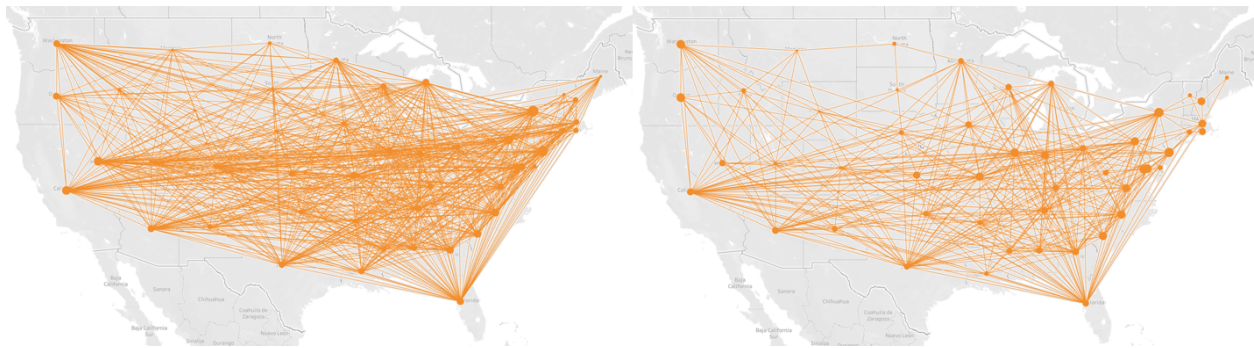
FIGURE 3: The inter-state flow connections of the week of March 2 (LEFT) and the week of April 6 (RIGHT). Each edge represents 10,000+ flow connecting two states. A significant reduction of the mobility flow is observed comparing the two weeks.
