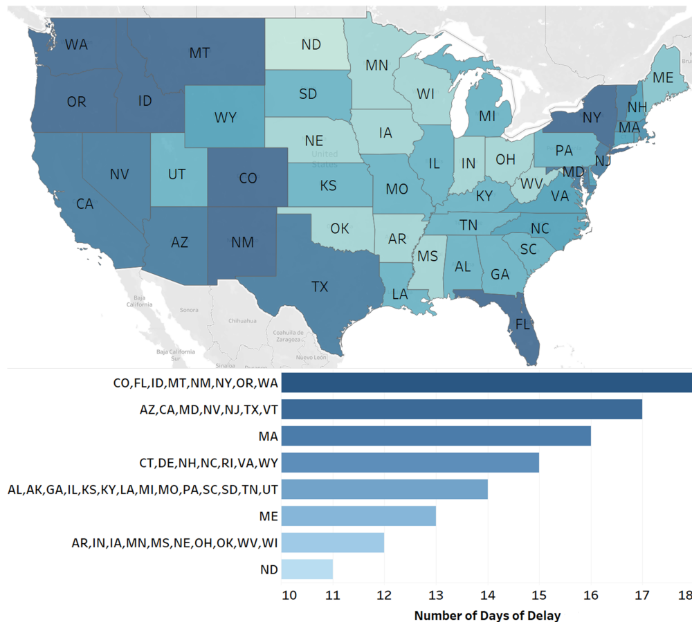
FIGURE 1: The number of days of delay reflected by Apple mobility data (2) to Google search data (15) for all states. The average delay of people’s mobility adjustment to their awareness of the pandemic is 14 days.
